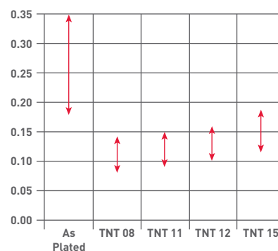
MacDermid Enthone friction control on zinc-nickel electroplate
